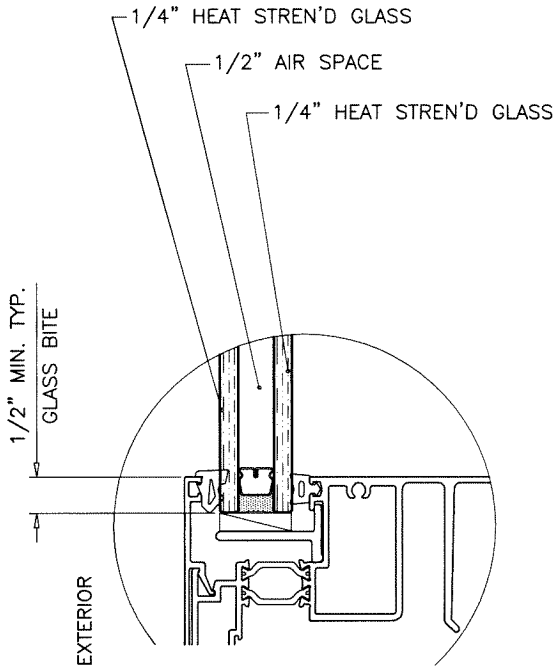
GLAZING DETAIL 1" OVERALL INSUL. GLASS
