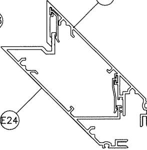
MULLION 'M3'
