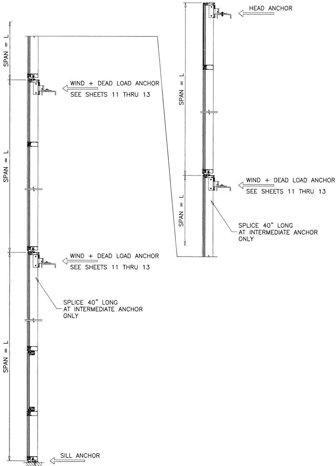
MULTIPLE SPANS
