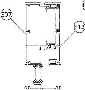
MULLION 'M1'
