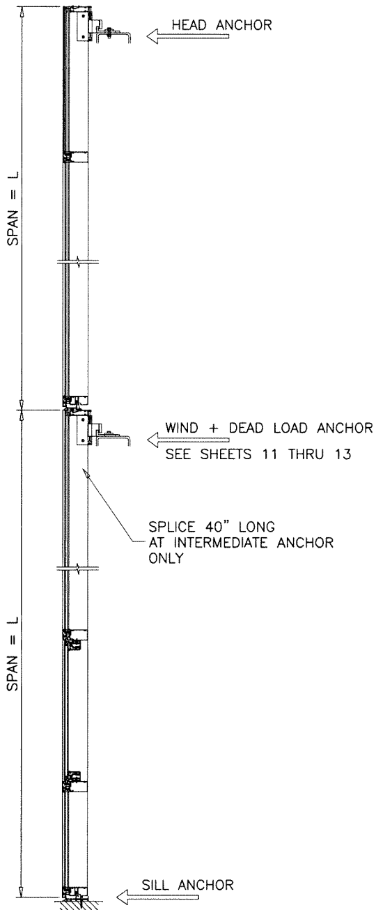
TWO SPAN
