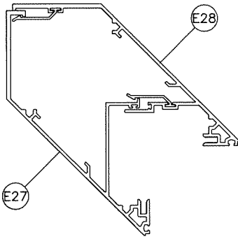
MULLION 'M4'
