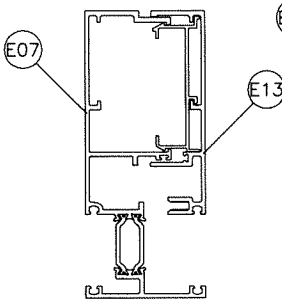
MULLION 'M1'
